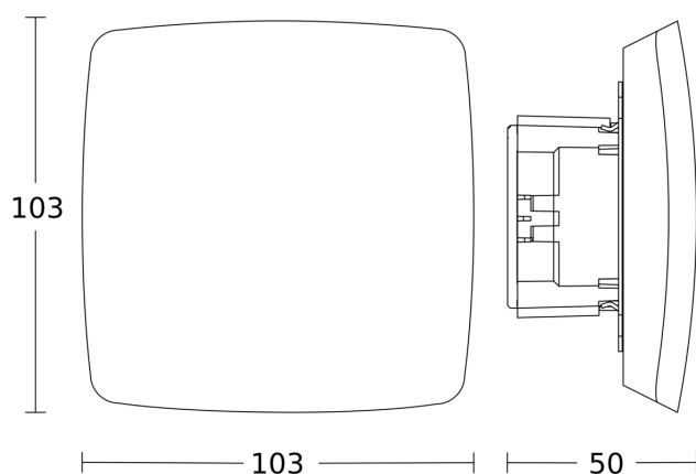
Dimension Drawing 1
